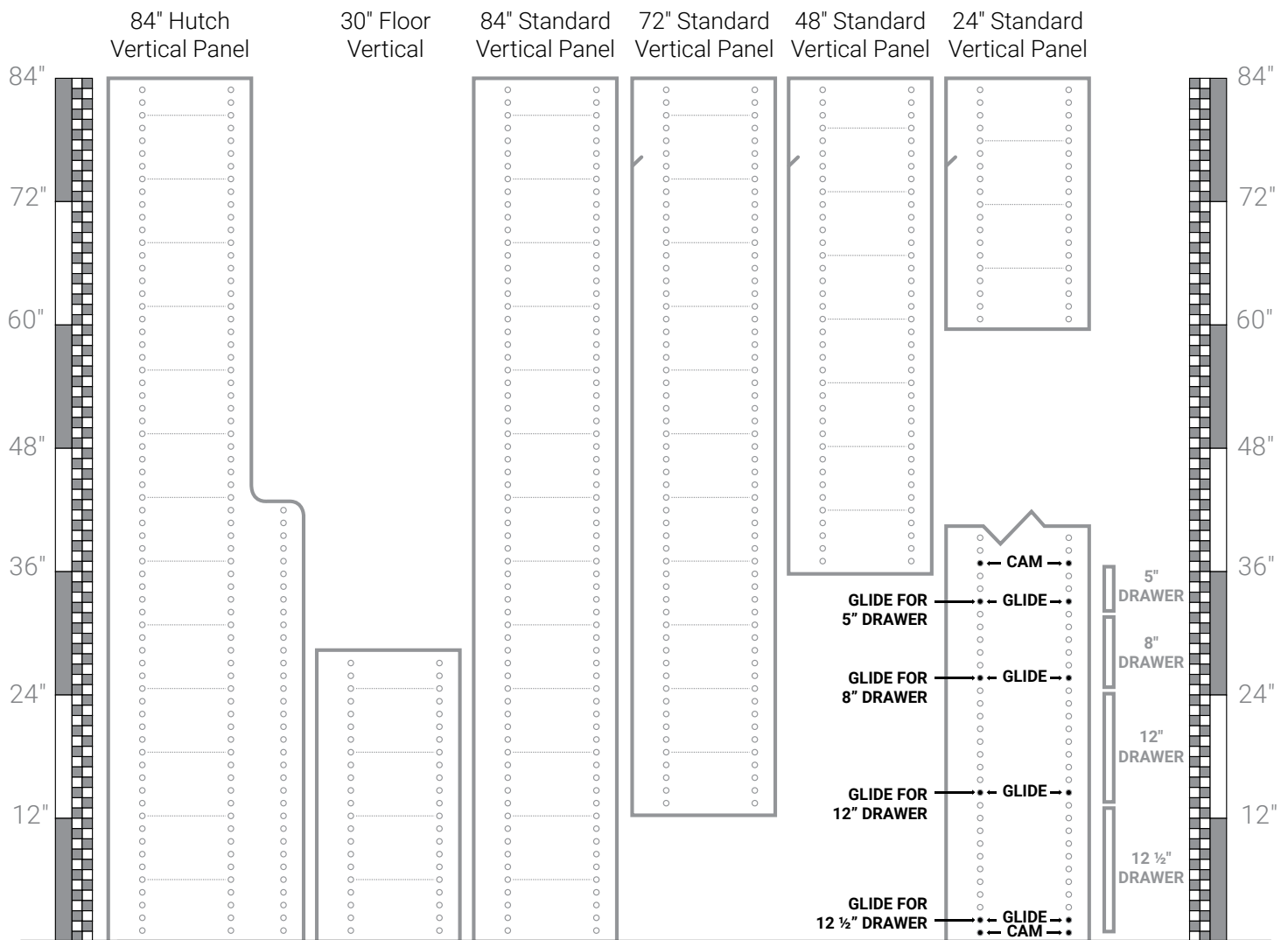
EXAMPLE PANEL MARKED FOR 4 DRAWERS AND 2 CAM SHELVES (BOTTOM RIGHT OF DIAGRAM)
